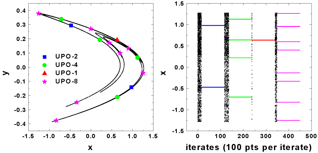
FIGURE 4. Hénon Map: The left panel shows the attractor with a number of embedded UPOs. The right panel shows the successive OGY control of UPOs of period 2, 4, 1, 8 for a_0 = 1.4, b_0 = 0.3 . The control is held for 10 000 iterates with \delta = 5 \times 10^{-3} and \delta a_{\max} = 10^{-2} a_0 .
