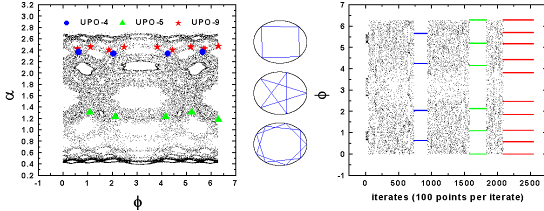
FIGURE 8. Cosine Billiard: (left) mixed chaotic (filled) and regular (open islands) phase space with embedded UPOs for \epsilon_0 = 0.3 ; (middle) MED controlled UPOs of period 4, 5, 9; (right) stabilized \phi variable of the corresponding UPOs held for 5 000 cycles each with \delta = 10^{-2} (1 cycle = 1 complete orbit).
